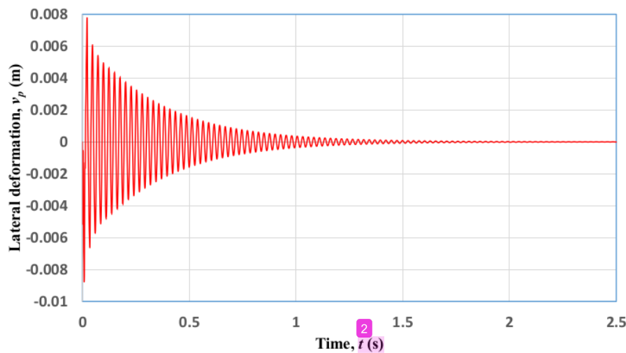
2 Figure 6. Time history response of the system
